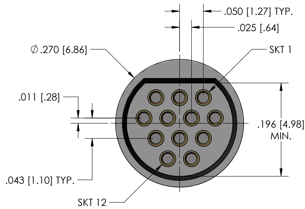
12 POSITION RECEPTACLE
