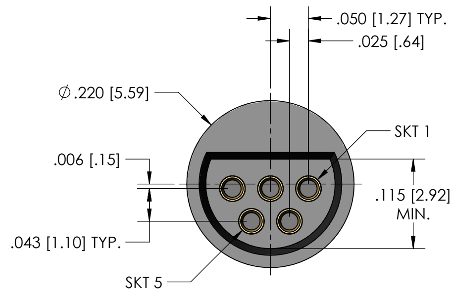
5 POSITION RECEPTACLE
