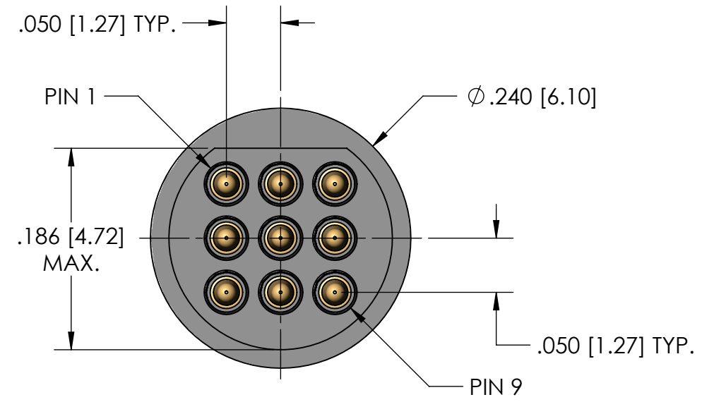
9 POSITION PLUG
