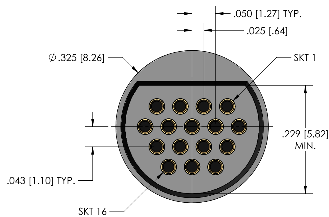
16 POSITION RECEPTACLE
