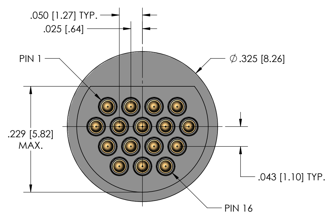
16 POSITION PLUG
