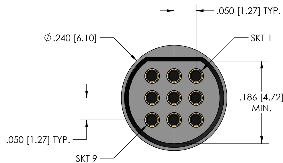
9 POSITION RECEPTACLE
