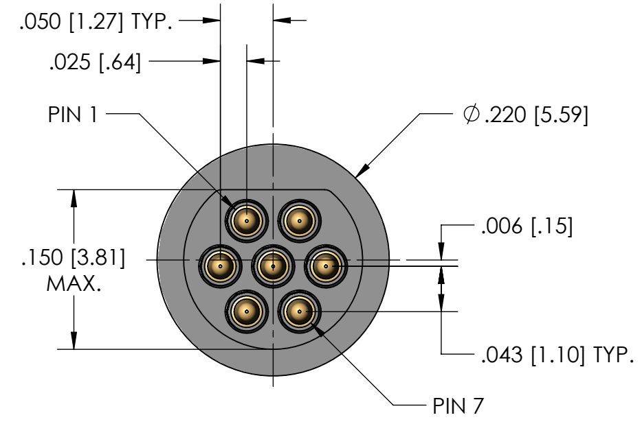
7 POSITION PLUG
