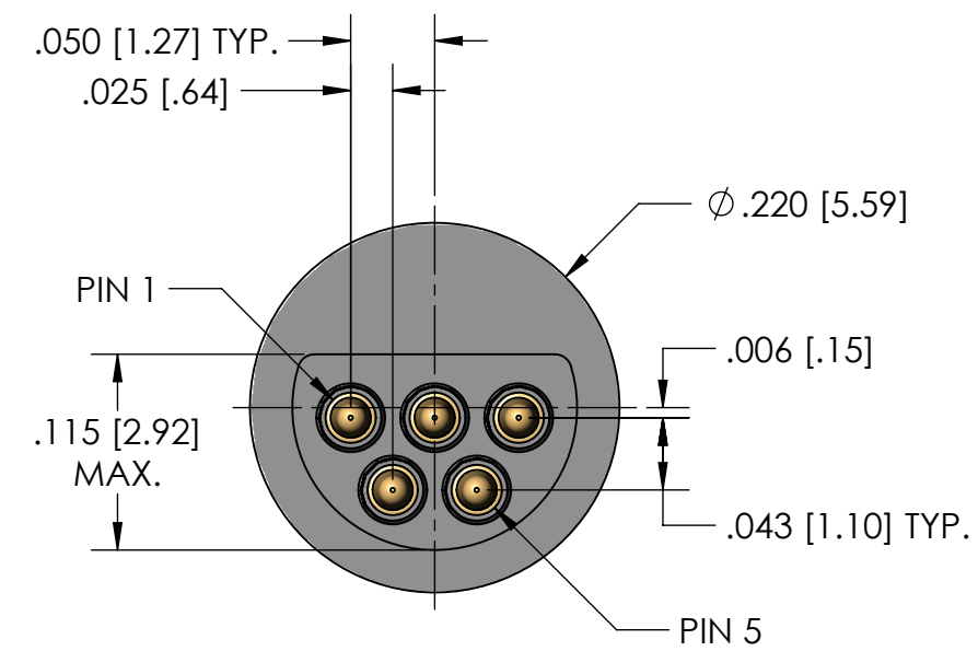
5 POSITION PLUG
