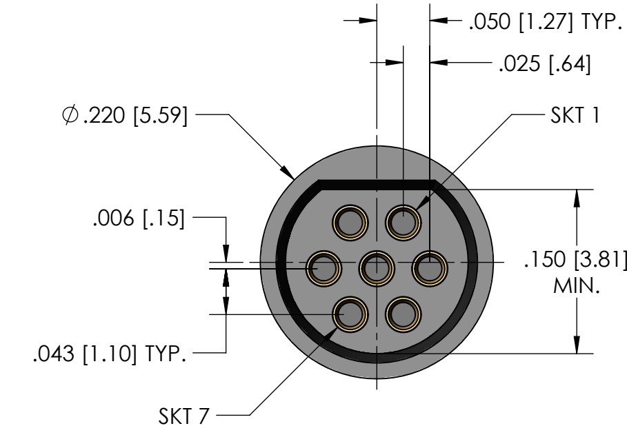
7 POSITION RECEPTACLE
