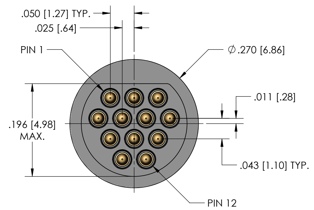
12 POSITION PLUG
